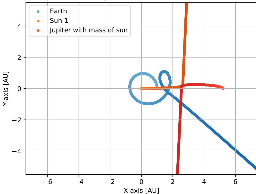
Map of motion of planets, 2nd sun with 1 solar masses
